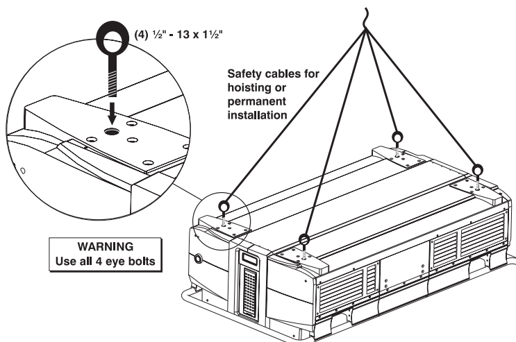
Figure 2-3. Safety Cables
