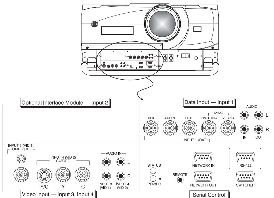
Figure 2-12. VistaGRAPHX 7000 Front Panel
