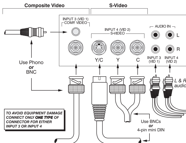
Figure 2-14. Composite and S-Video Inputs
