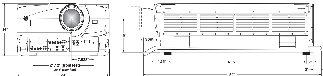
Figure 5-1. Projector Dimensions
