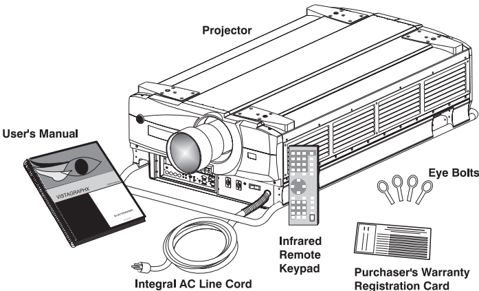
Figure 1.2. VistaGRAPHX 7000 System Components (with Lens Added)
