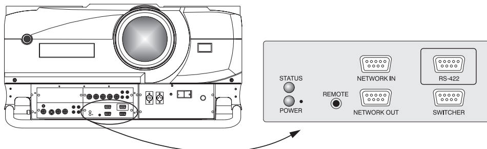
Figure 2-16. Serial Port Connections — RS-232 or RS-422
