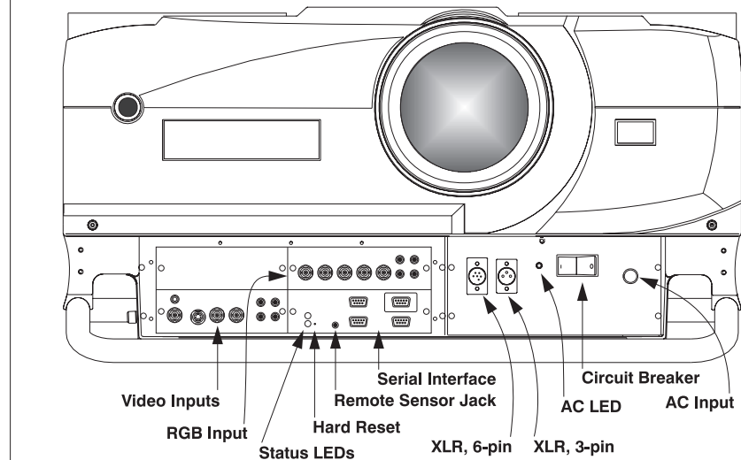
Figure 3-2. Detail of Front Panel
