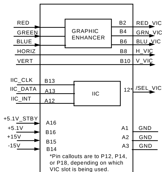
Figure 2-6. Graphics Enhancer RGB VIC I/O
