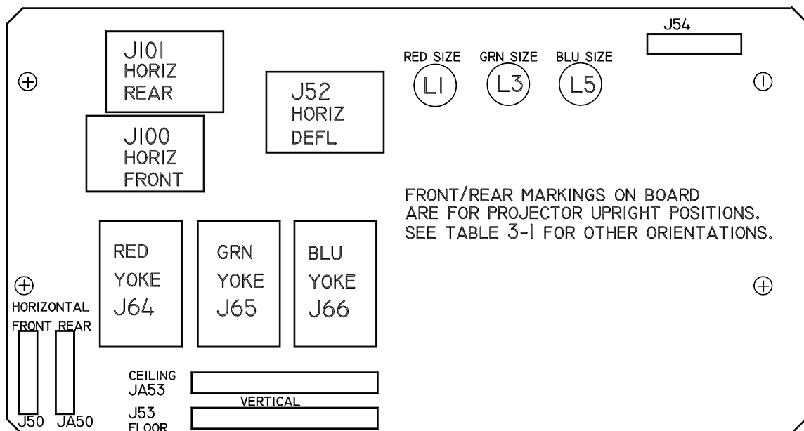
Figure 4-13. Scan Reversal PCB.
