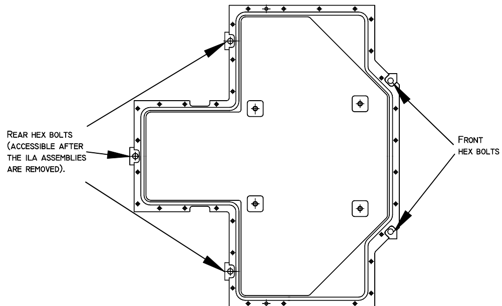
Figure 4-17. Dichroic Mirror Assembly.
