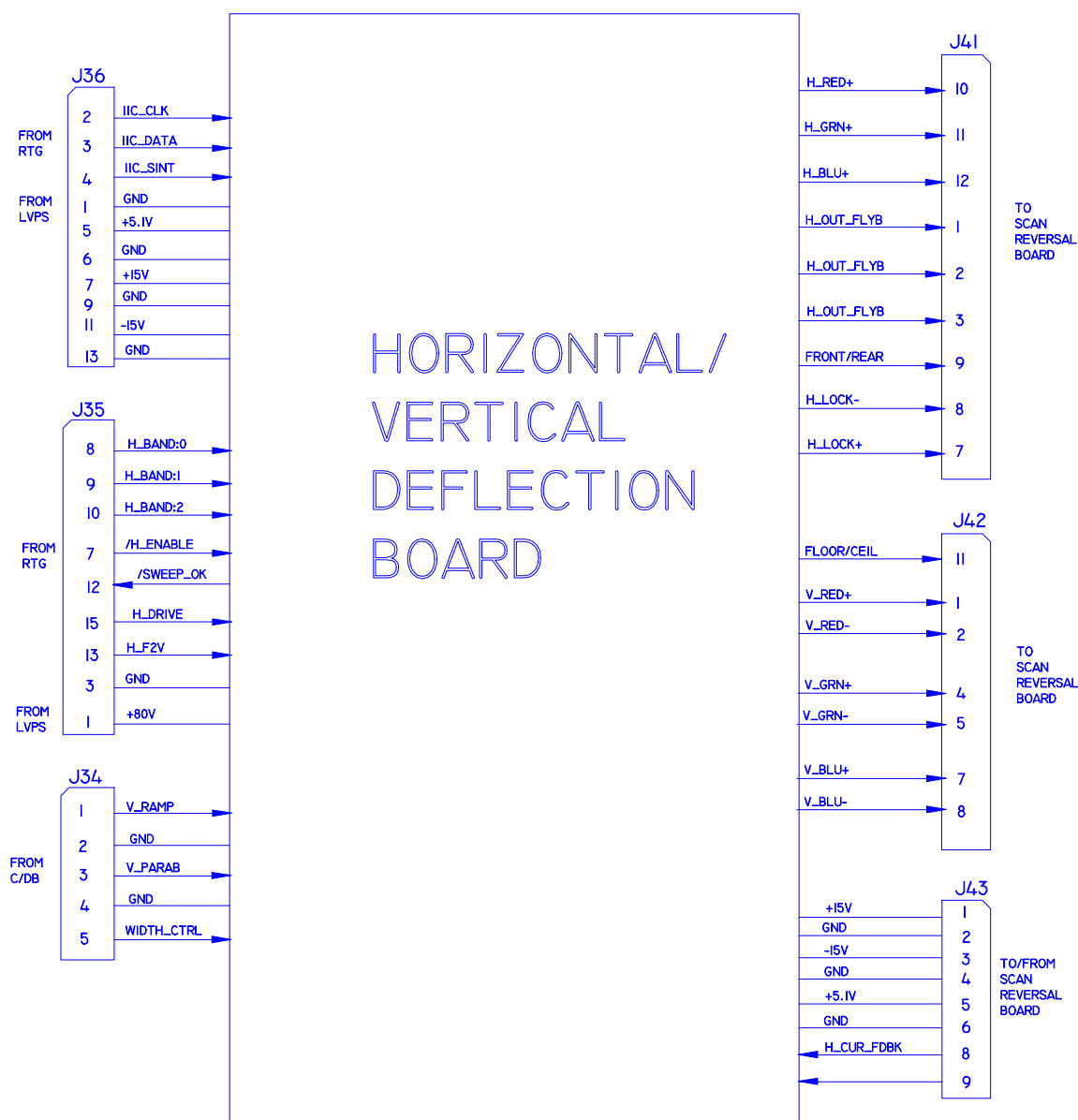
Figure 2-14. Horizontal/Vertical Deflection PCB I/O Diagram.
