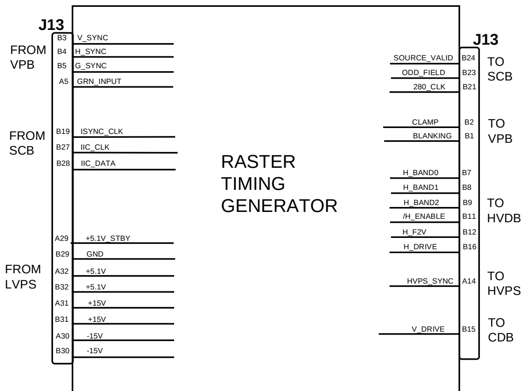
Figure 2-13. Raster Timing Generator, Input/Output Diagram.
