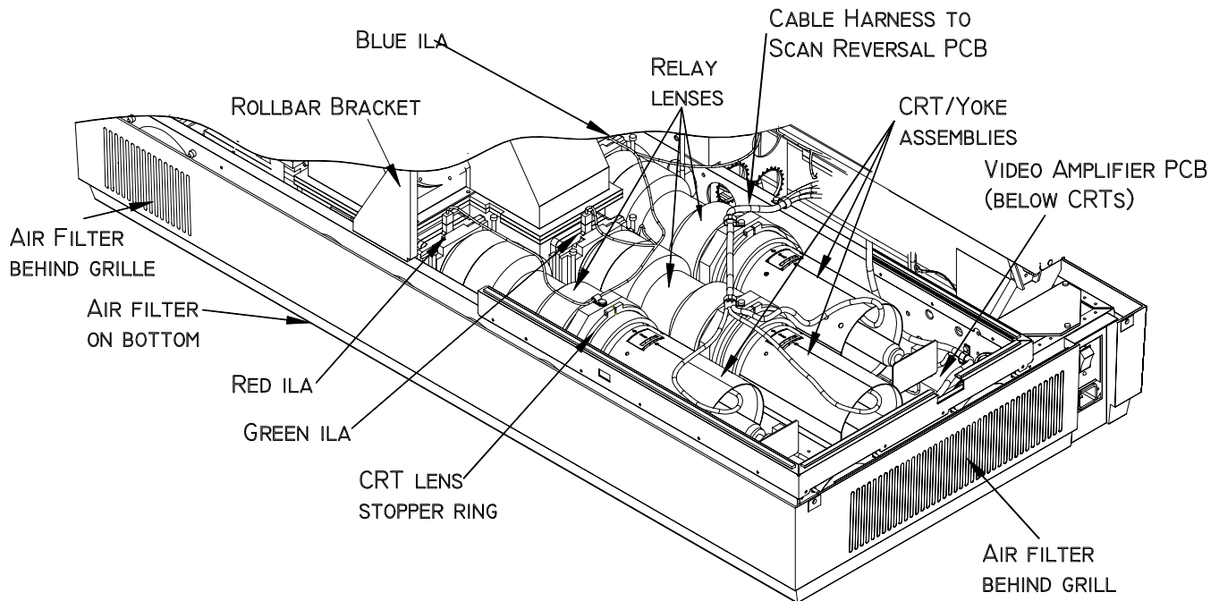
Figure 3-2. View of CRTs, Relay lenses and ILA® Assemblies.
