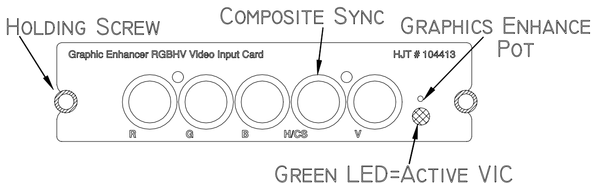
Figure 3-15. Graphic Enhancer Video Input Card.
