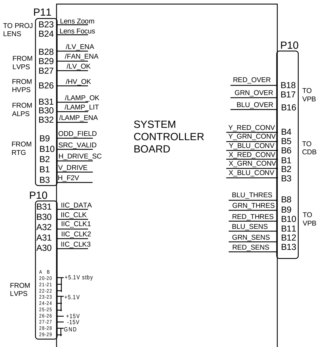
Figure 2-12. System Controller Board, Block Diagram.
