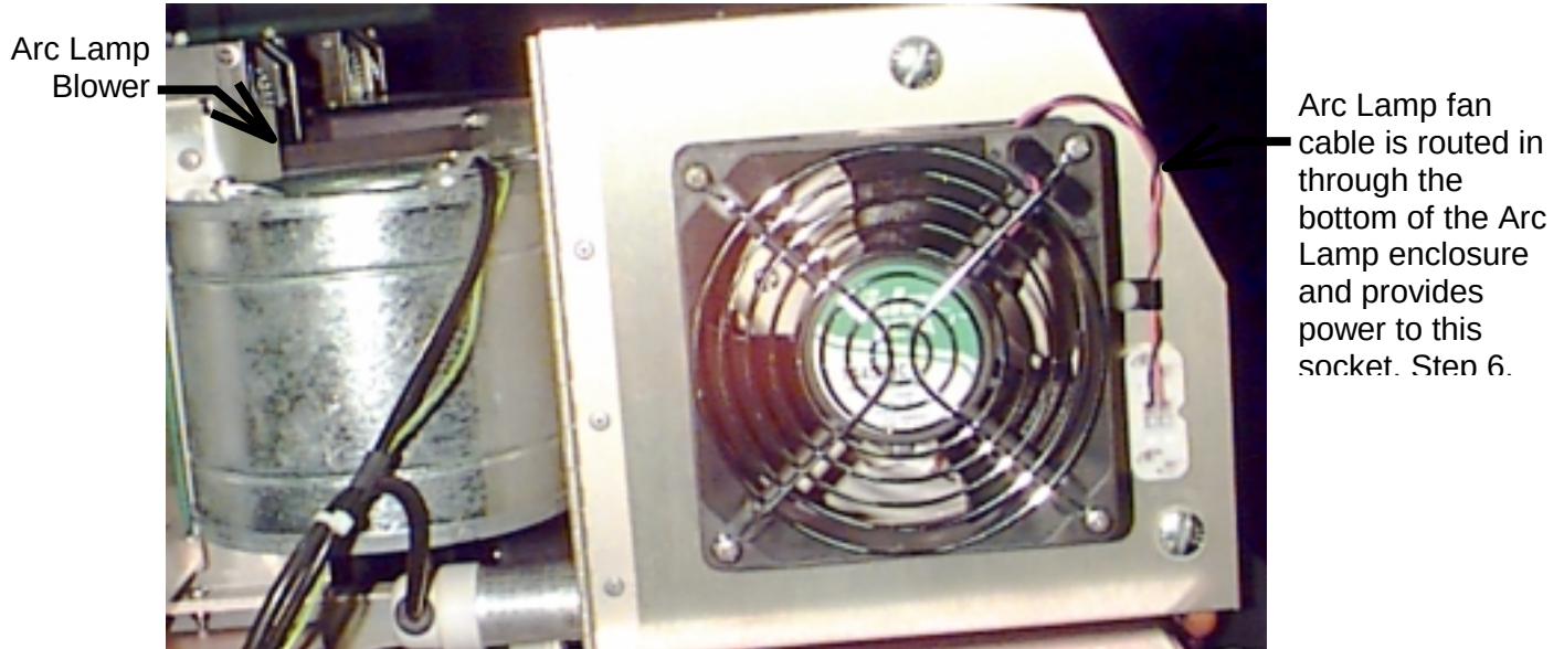
Figure 4-3. Arc Lamp Assembly
