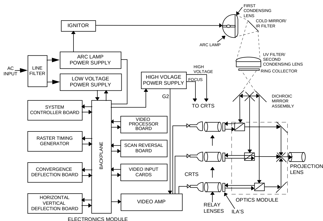
Figure 2-2. Model 230 System Block Diagram
