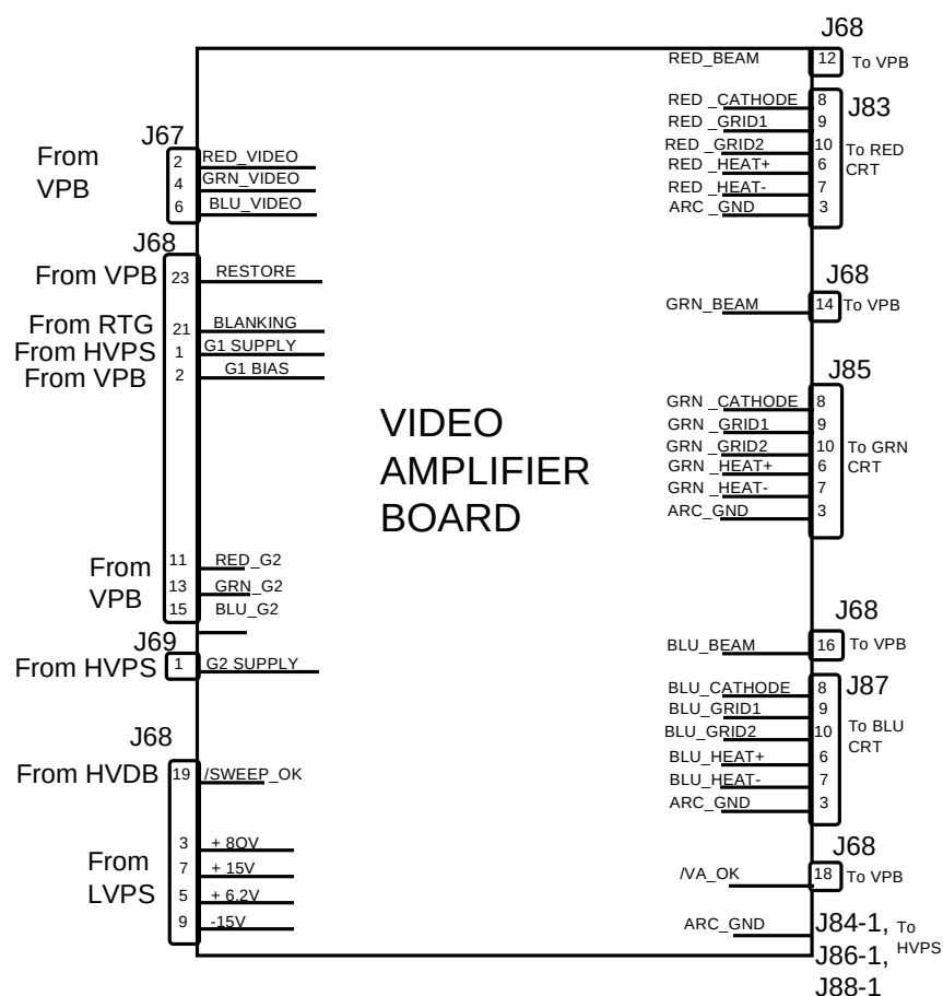
Figure 2-11. Video Amplifier PCB, Block Diagram.
