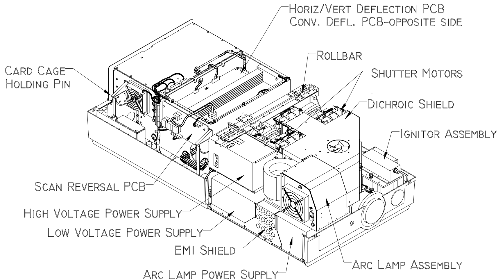
Figure 3-1. Major components of the Model 230 Projector.
