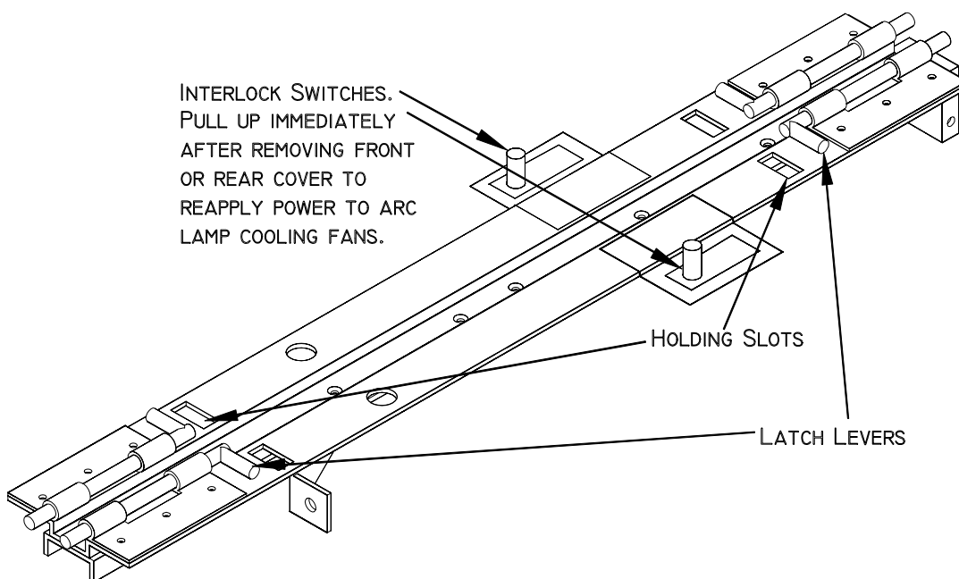
Figure 4-2 Rollbar Assembly.
