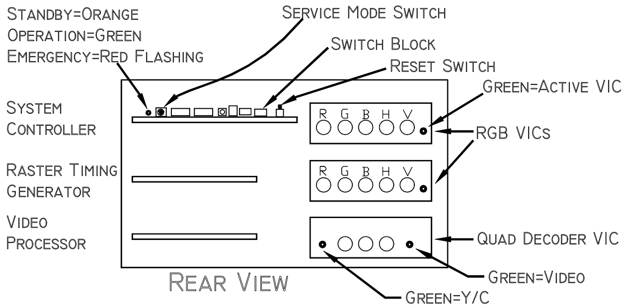
Figure 5-1. Projector rear with cover and rear panel off.
