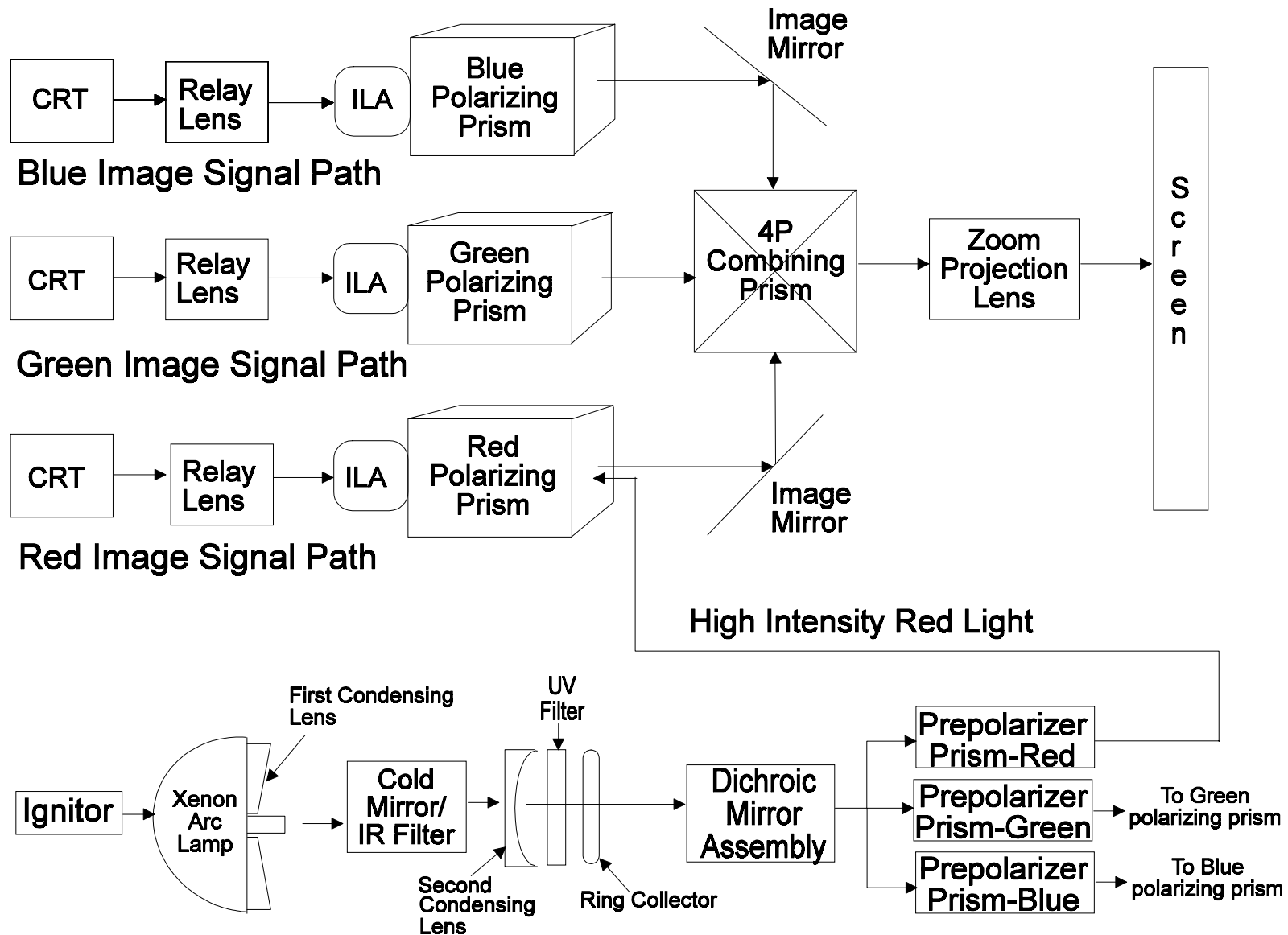
Figure 2-1. Optical System Block Diagram
