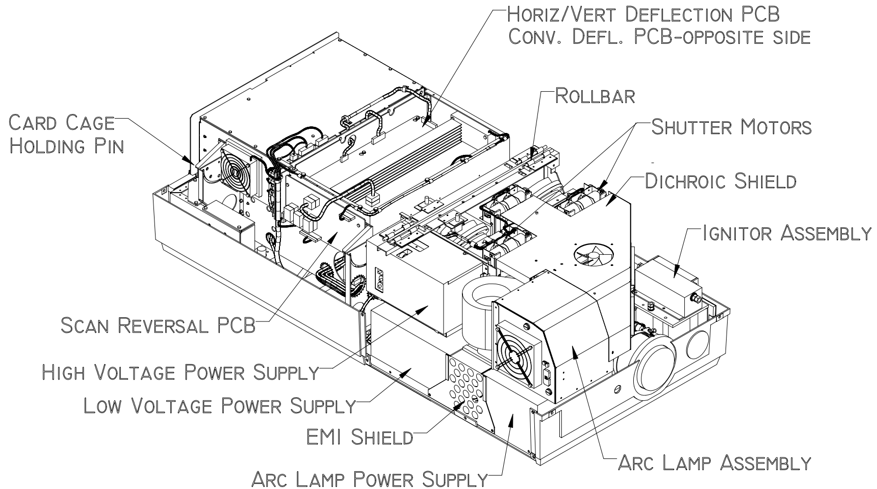
Figure 4-1. Major components of the Model 230 Projector.
