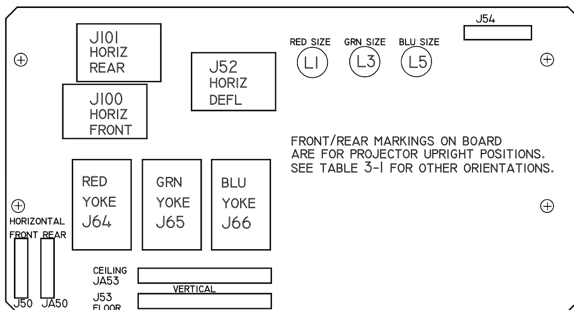
Figure 3-13. Scan Reversal Board.
