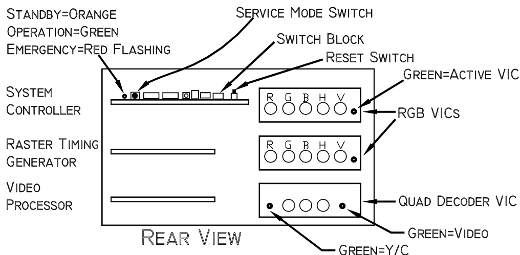
Figure 4-9. Projector rear with cover and rear panel off.
