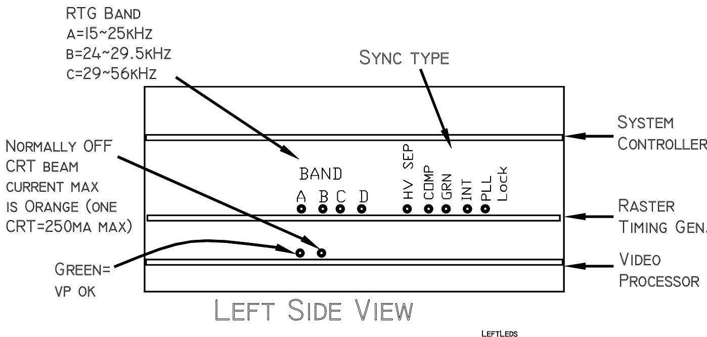
Figure 5-2. Left side of projector with rear cover off.
