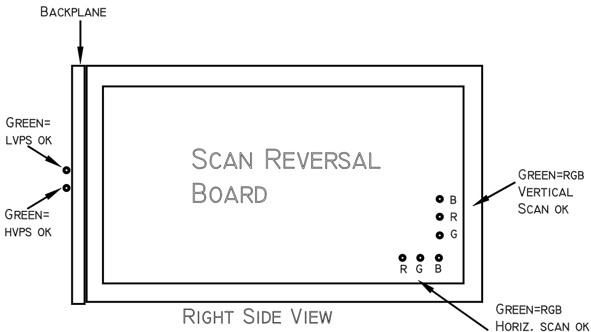
Figure 5-3. Right Side of projector with rear cover off.
