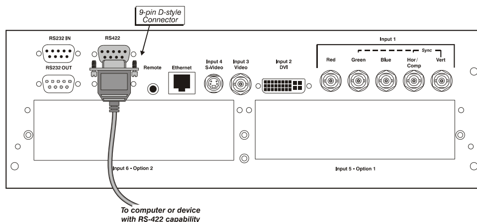
Figure 2.11. Connecting RS422
