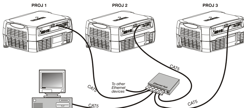
Figure 2.13. Ethernet Network
