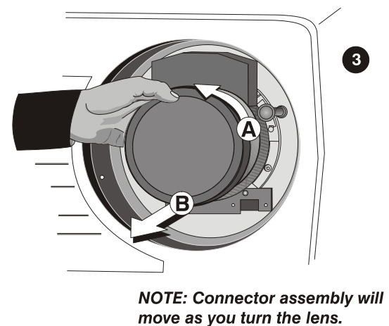
Figure 4.12. Rotating the Lens
