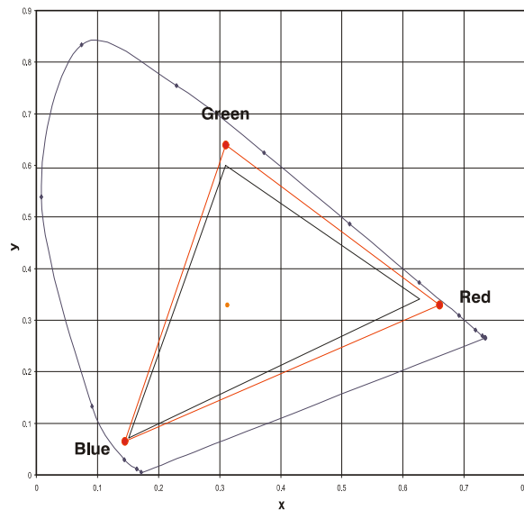
Figure 3.11. CIE 1931 Chromaticity Diagram (without Yellow Notch Filter)
