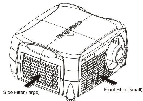
Figure 4.7. Filter Location
