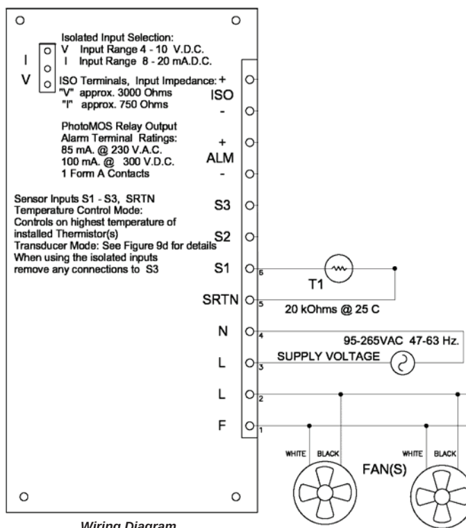
Wiring Diagram
