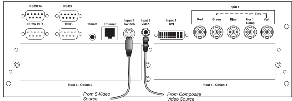
Figure 2.9 Connecting Composite or S-Video sources
