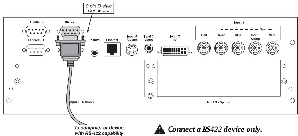
Figure 2.11 Connecting RS-422
