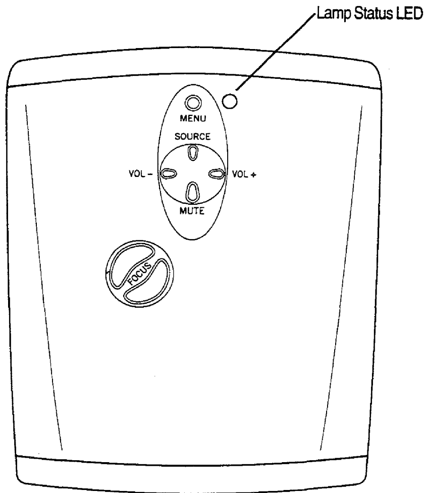
Figure 5: Keypad Controls
