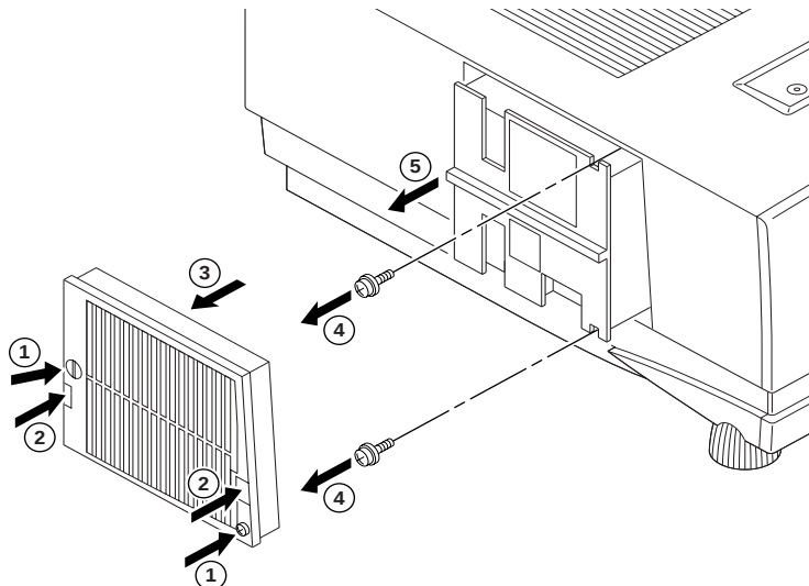
Figure 6.1 Lamp Module
