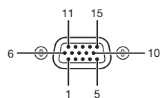
COMPUTER IN, MONITOR OUT (Mini D-SUB 15-pin)
