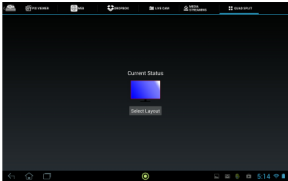
Android screen
