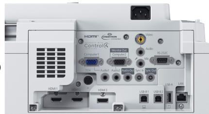
Additional USB-A port on side of projector
