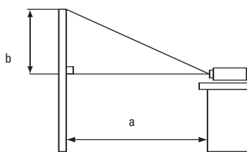
a: Projection Distance b: Lens centre to the higher edge of the screen
