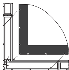
Cineperm Truss-Style Construction (very large sizes only)
